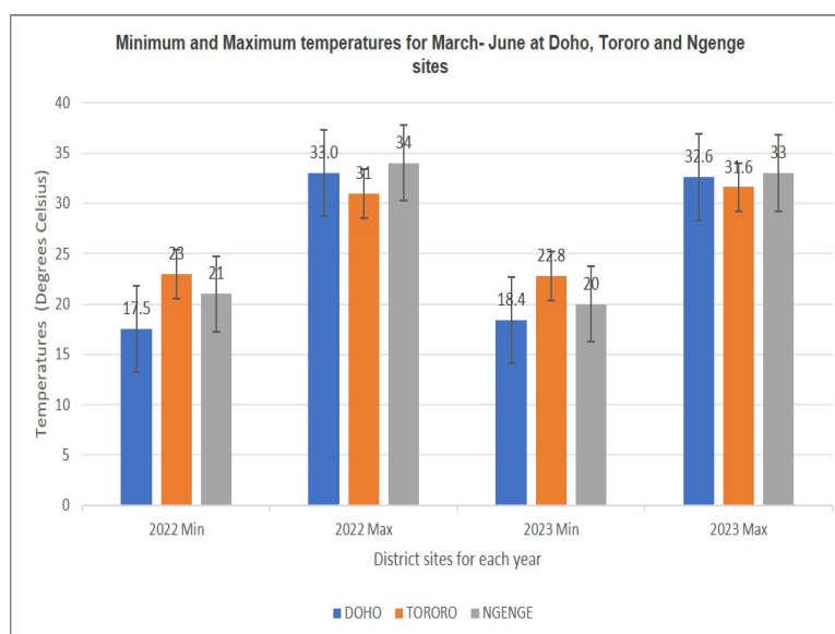
Figure 2: Minimum and maximum Temperatures at Doho, Tororo and Ngege sites during 2022 & 2023
